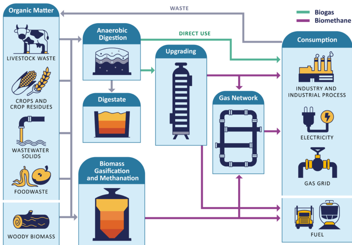
FIGURE 6-2. BIOGAS PATHWAYS 168
